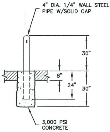
PIPE BOLLARD DETAIL
