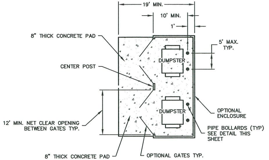
DOUBLE DUMPSTER ENCLOSURE
