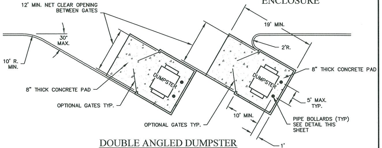
DOUBLE DUMPSTER ENCLOSURE
