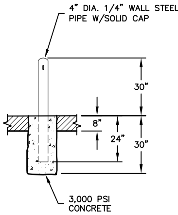
PIPE BOLLARD DETAIL
