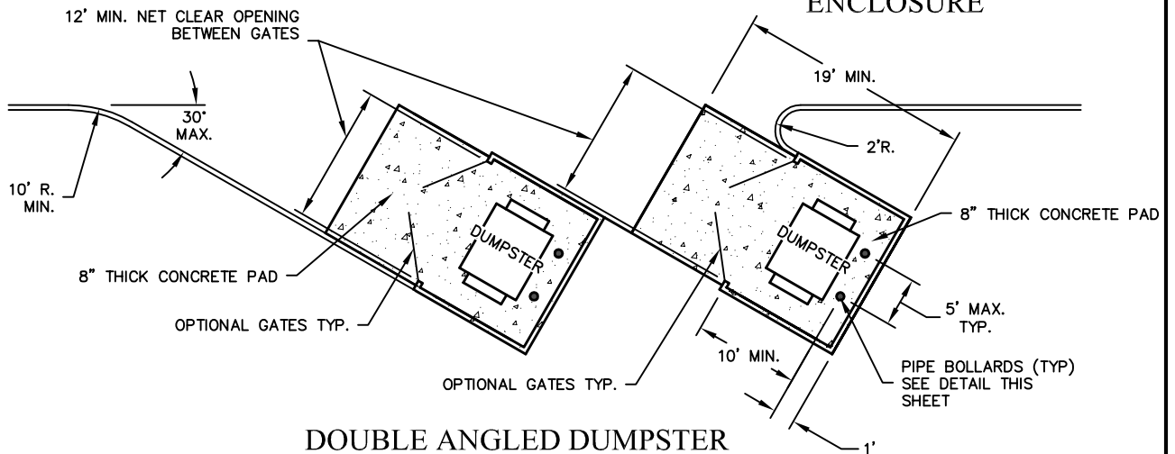
DOUBLE DUMPSTER ENCLOSURE
